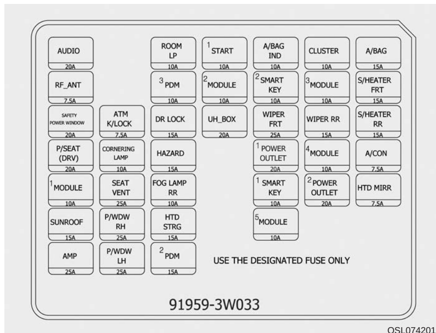
Instrument panel fuse panel
